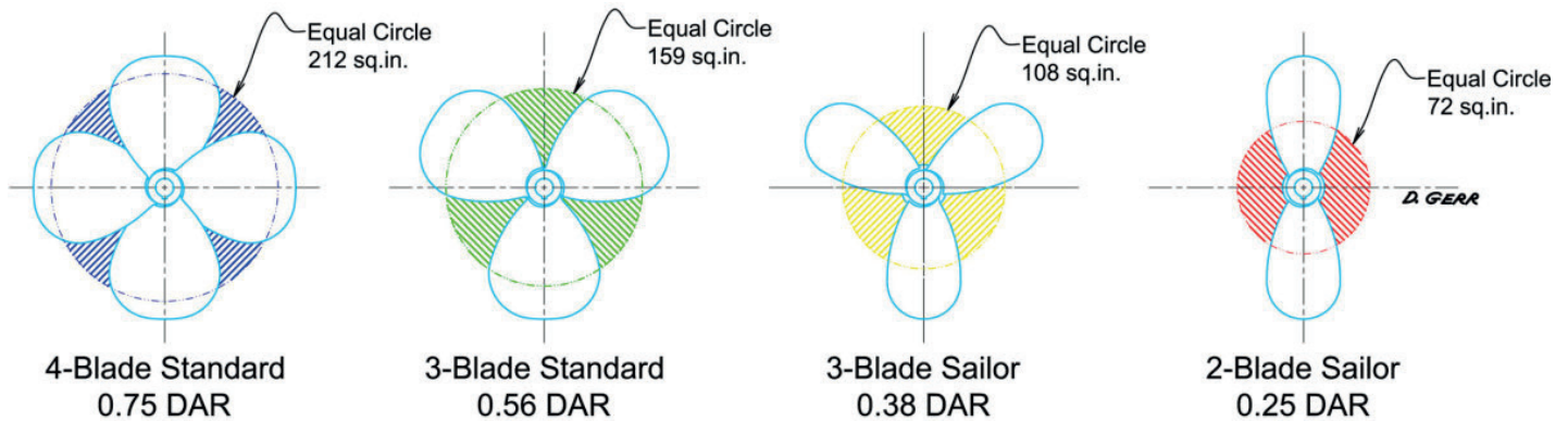
Propeller Blade Areas Compared - All 19-in. Diameter
